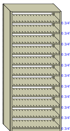
R2 36"W x 9"D H=85 1/4"
