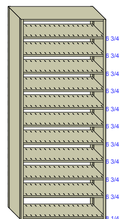
R4 36"W x 9"D H=85 1/4" SysH=90 3/4"
