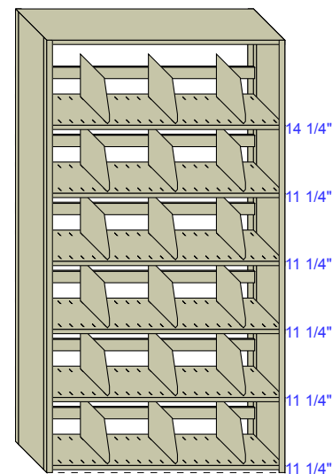
R2 42"W x 12"D H=76 1/4" SysH=83 3/4"
