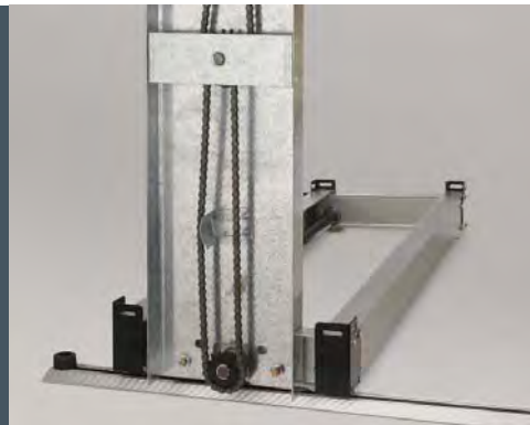
MECHANICAL END PANEL UTILIZES A FULL-LENGTH DRIVESHAFT TO ENSURE SIMULTANEOUS MOVEMENT.
